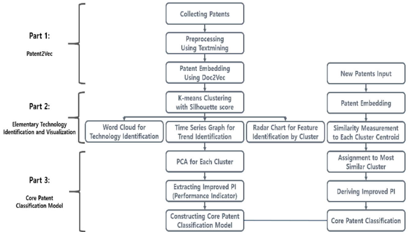
Fig. 1. Proposed methodology
