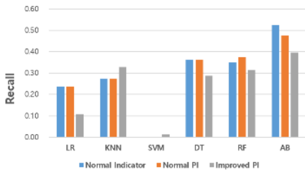
Fig. 10. Recall by input variables and models
