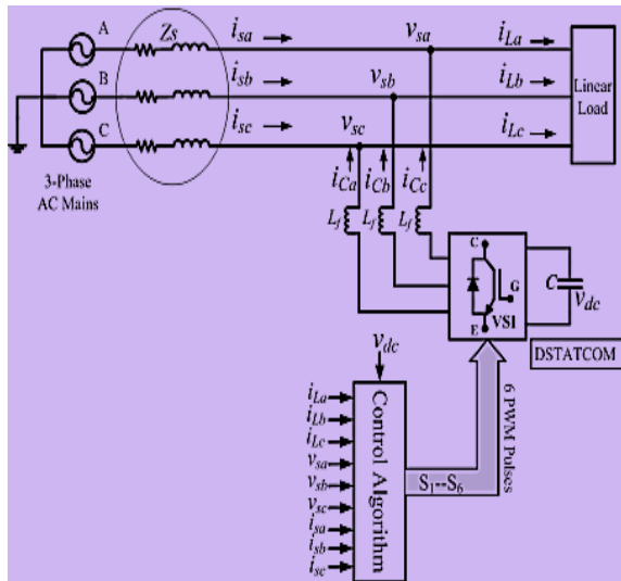
Fig. 1. Schematic configuration of DSTATCOM
