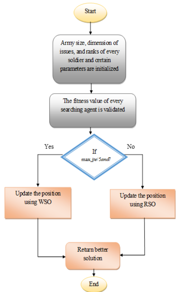
Fig 2. The ICWRS model's flowchart In essence, ICWRS represents a groundbreaking strategy
