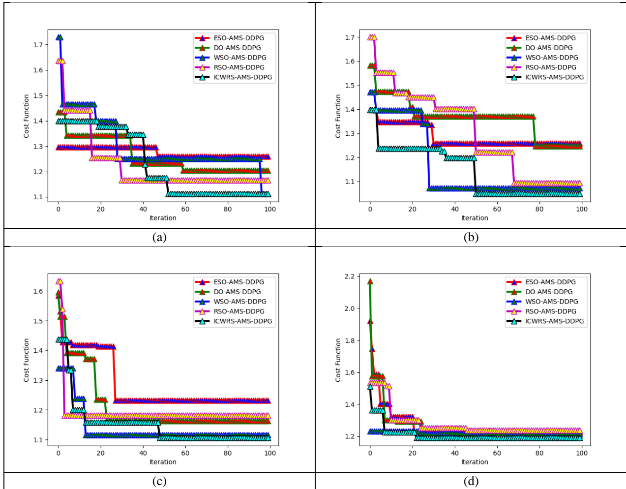
Fig 3. Demonstrates how the cost function is used to validate the suggested cloud-based job scheduling and virtual machine migration framework algorithmically in the following configurations: Configurations 1, 2, 3, and 4 are listed in order of preference.
