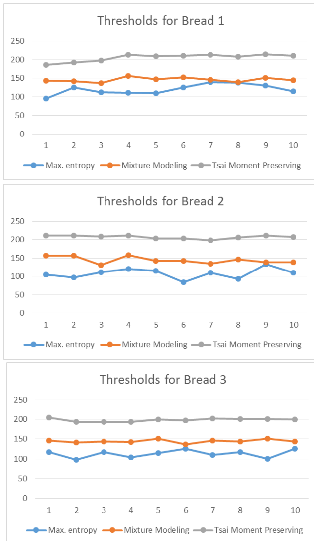
Figure 4. Threshold values for 10 images
