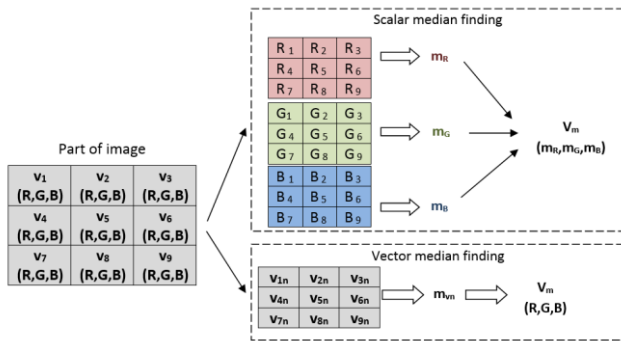
Figure 3. Scalar and vector determining the median value
