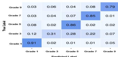
Fig 11: Confusion matrix
