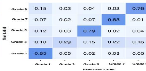
Fig 11: Confusion matrix
