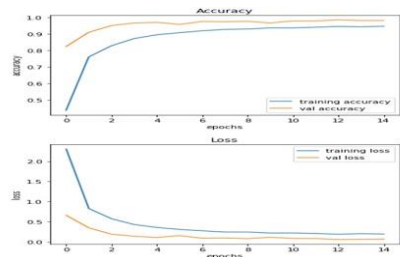
Fig 12: Train, Test Accuracy, and Loss
