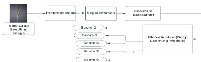
Fig 3: Workflow of proposed methodology
