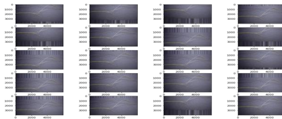
Fig 7: Data Augmentation
