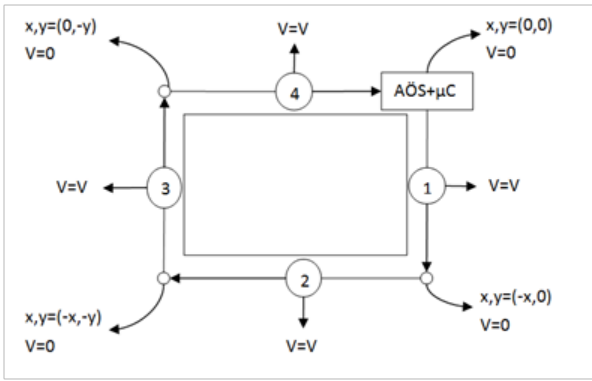
Figure 9. Plotting rectangular shape with IMU and microcontroller
