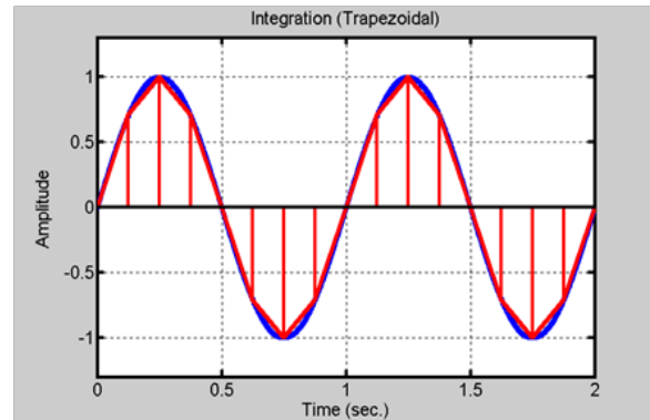
Figure3. Trapezoidal integration
