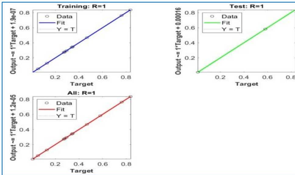
Fig. 4 Calculation results Matlab: training and test with R
