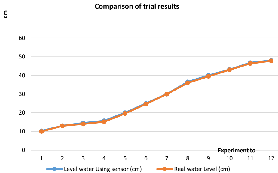
Fig. 2 Comparison of Water Level Sensor Results with Condition real
