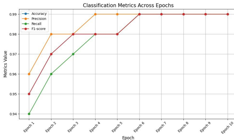
Fig 6: Classification with HFWDR
