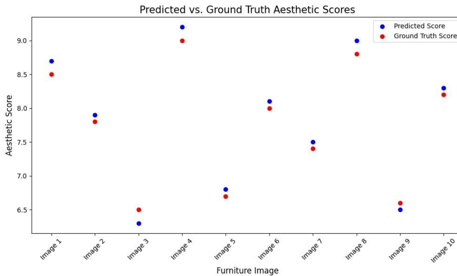
Fig 5: Aesthetic Score
