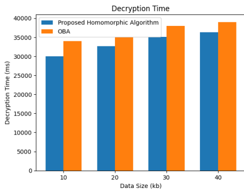
Figure 6: Decryption Time
