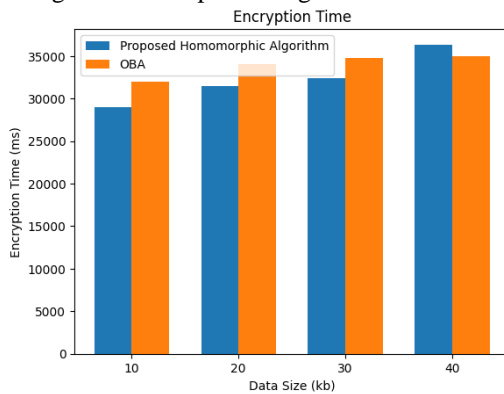
Figure 7: Encryption Time
