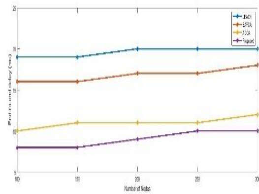
Fig 7: End-to-end delay
