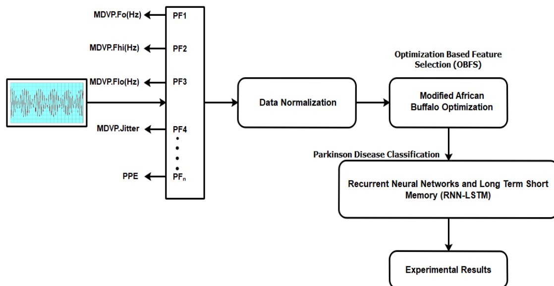
Fig 1. PD Patients Identification/Classification System Model
