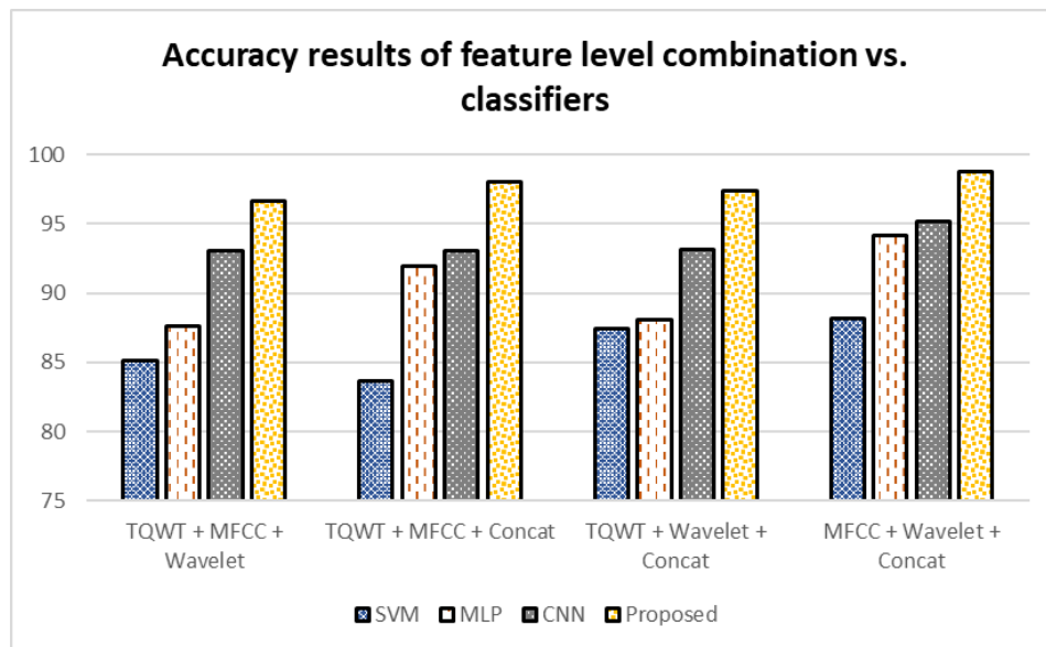
Fig 4. Results of feature level combinations vs. classifiers in terms of accuracy
