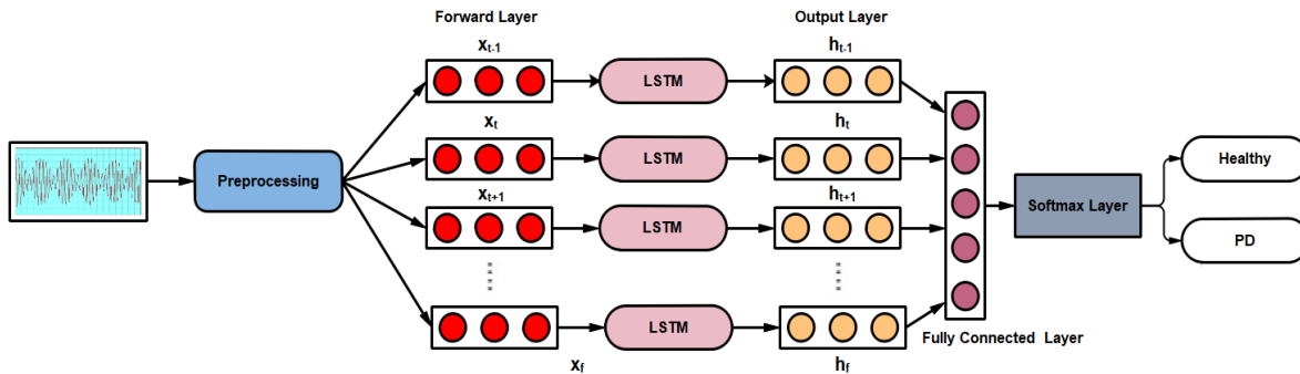
Fig 2. Proposed RNN-LSTM classifier for PD diagnosis
