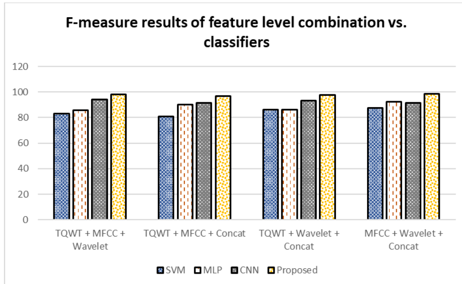
Fig 5. F-measure outcomes for a combination of feature levels versus classifiers.
