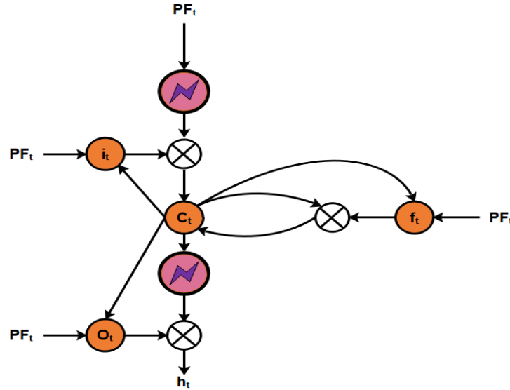
Fig 3. LSTM cell
