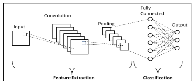
Fig. 1. CNN network architecture [12]
