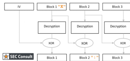
Fig. 3(b) : Cryptographic vulnerabilities
