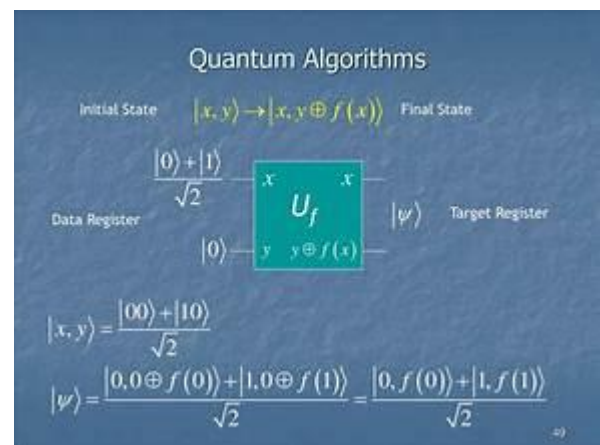
Fig. 2(c): Quantum Algorithm
