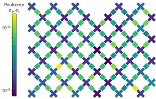
Fig. 5(d) : Heat map showing single- (e1; crosses) and two-qubit (e2; bars) Pauli errors for all qubits operating
