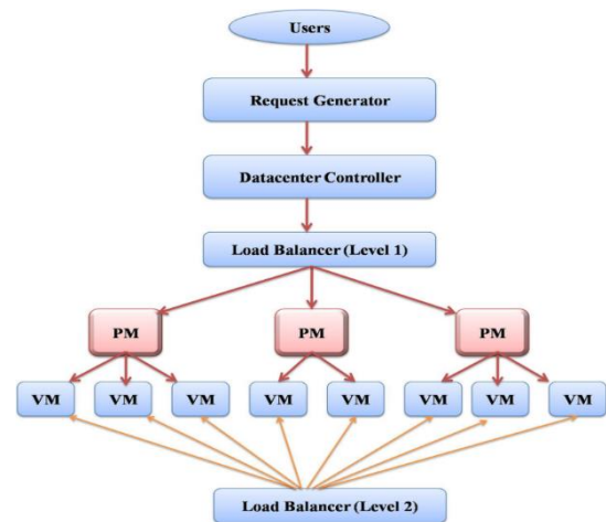
Fig 3: Load Balancer operations in VM level
