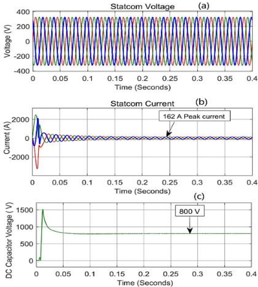
Fig 5. Analysis of Output Characteristics for Grid Stability
