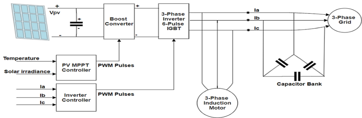
Fig 3. Fixed capacitor PV grid connected schematic
