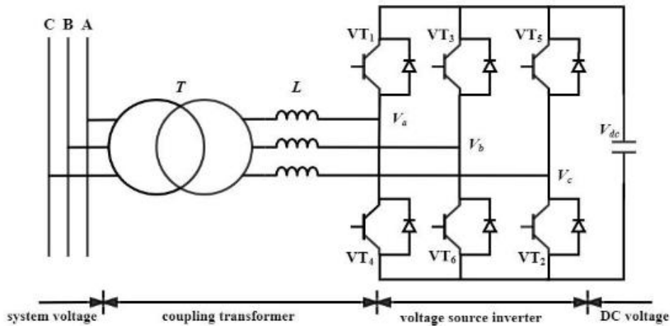
Fig 1. Fundamental Architecture of STATCOM
