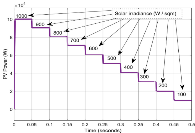
Fig 2. Optimizing PV Array Power Output in the Face of Solar Irradiance Fluctuations: A Controller Approach
