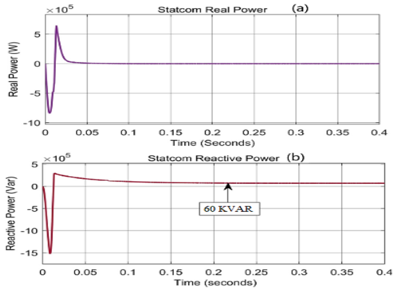
Fig 4. a) Active, b) reactive Power Supply by STATCOM
