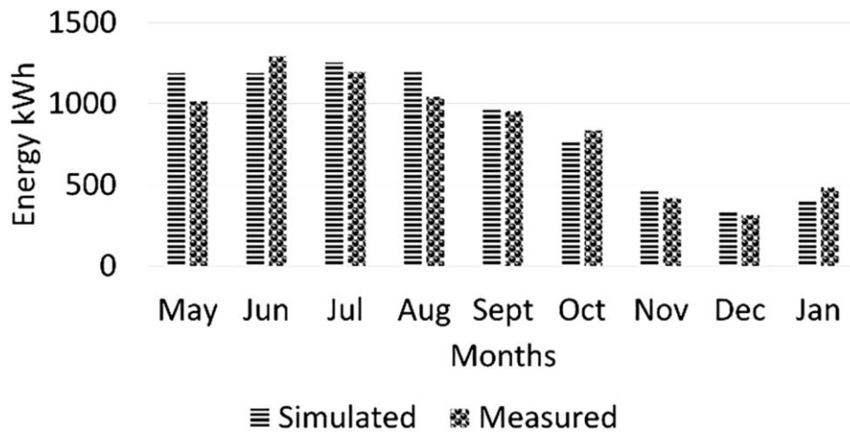
Fig 4. Comparison of Simulated and Observed Solar Energy Production
