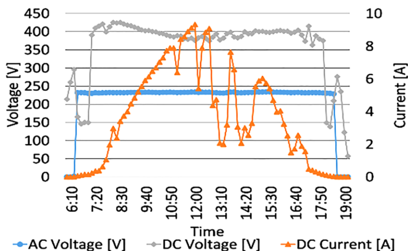
Fig 3. Analyzing Voltage and Current Diagrams: Solar Inverter Performance on a Cloudy Day
