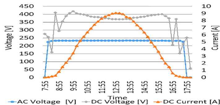
Fig 2. Solar Inverter Performance on a Sunny Day: Voltage and Current Diagrams
