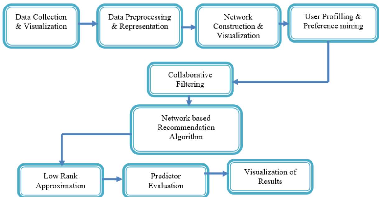
Fig. 1. Methodology for Link Data Mining
