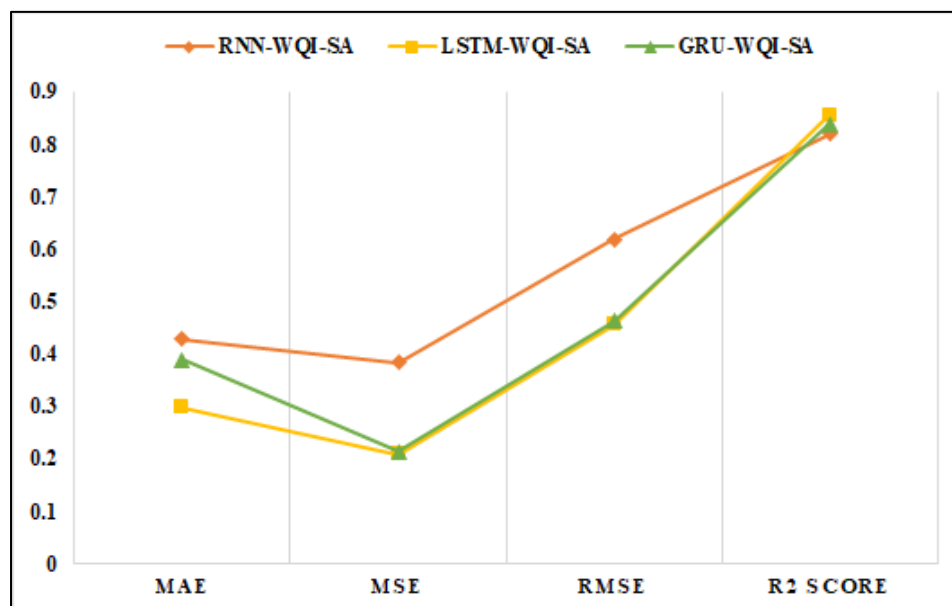
Fig.3. Prediction Performance of all Three WQI Models
