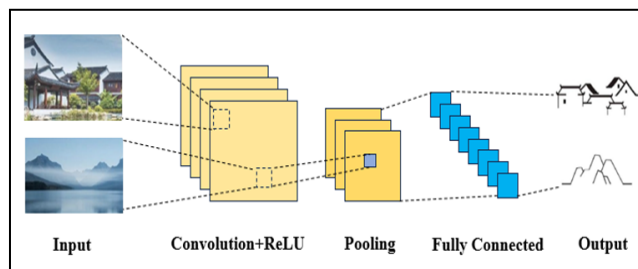
Fig. 4 Feature extraction and recognition framework of regional cultural elements
