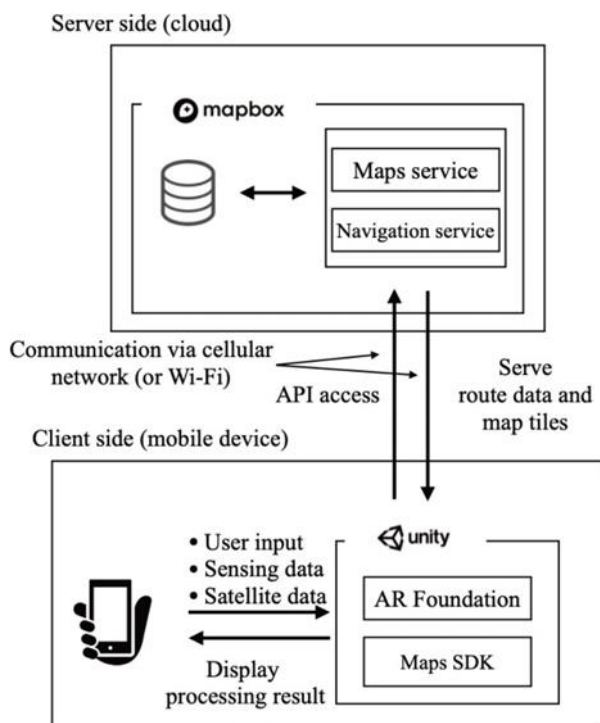
Figure 4. Overview of the system. Source: (14)
