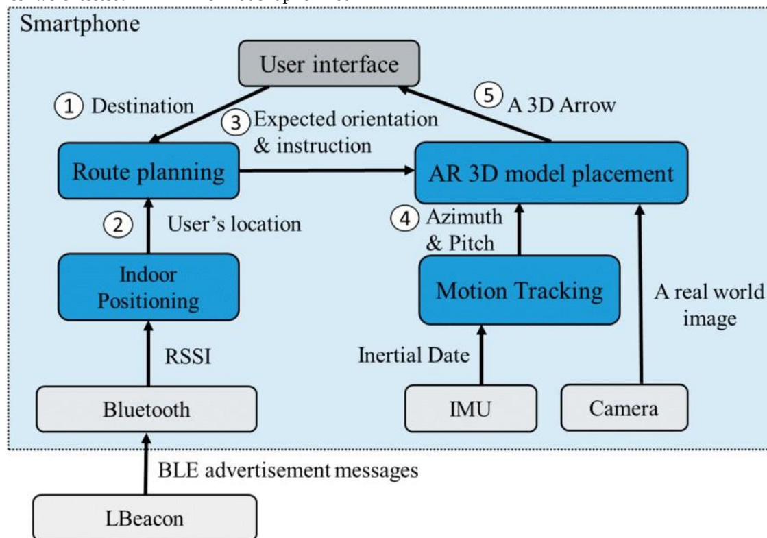
Figure 2. ARBIN system architecture. Source: (8)
