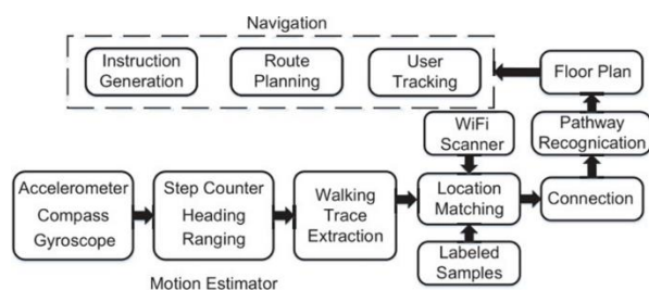
Fig 3. Architecture of the IndoorWaze system. Source: (9)
