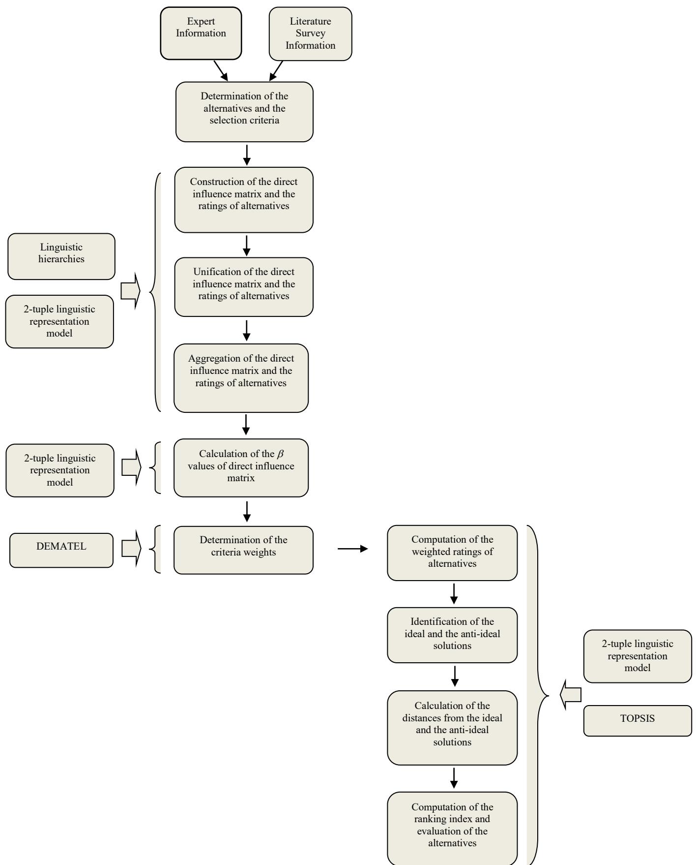
Fig. 1 Illustration of the proposed fuzzy decision making algorithm.
