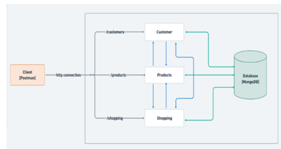
Fig. 1: Monolithic Architecture
