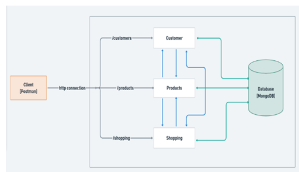
Fig. 2: Microservices Architecture
