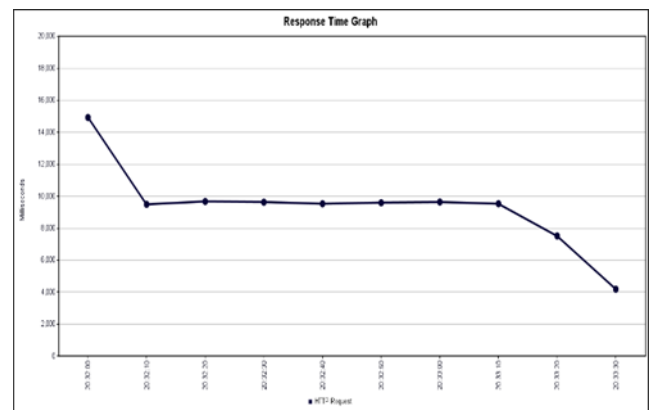
Fig. 4 Microservice Response Time Graph with 10,000 samples
