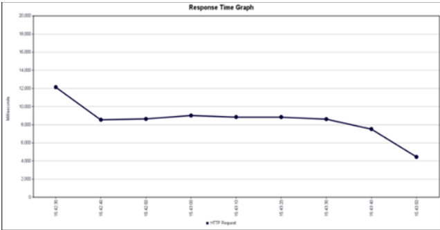
Fig. 9: Microservice Response Time Graph using Single MongoDB Instance
