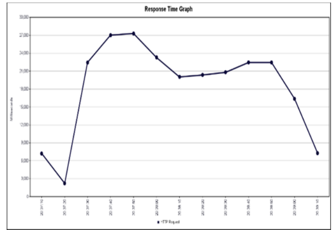
Fig. 3 Monolithic Response Time Graph with 10,000 samples
