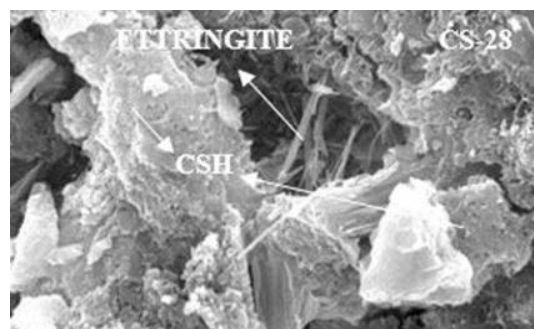
Fig 6 SEM Image for M-1 after 28 days Curing
