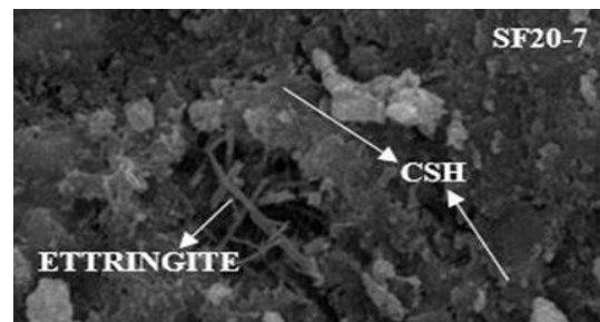
Fig-5 SEM Image for M-5 after 7 days Curing
