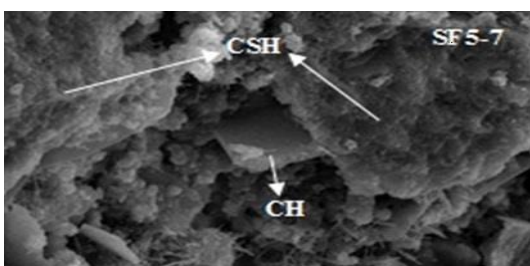
Fig-2 SEM Image for M-2 after 7 days Curing
