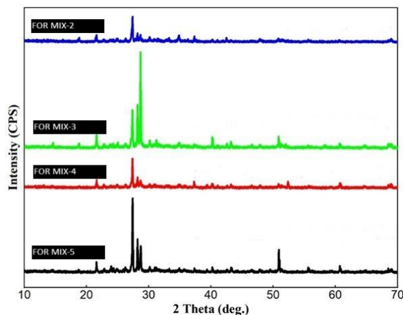
Graph-1 X-Ray Diffraction Observations
