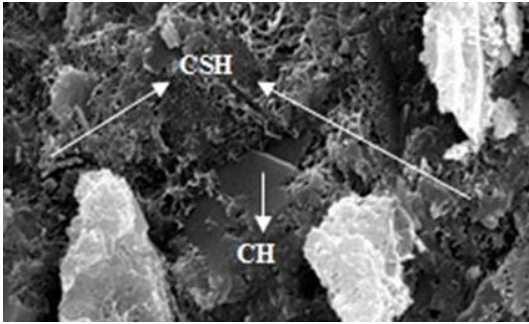
Fig-7 SEM Image for M-2 after 28 days Curing
