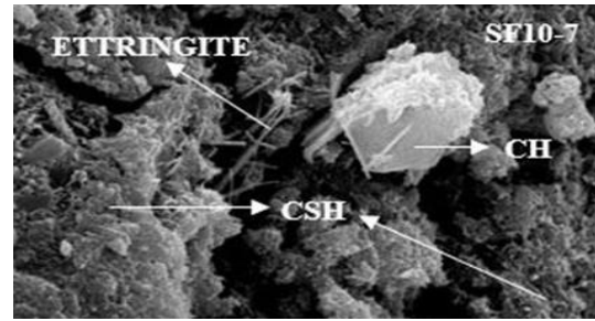
Fig-3 SEM Image for M-3 after 7 days Curing
