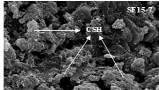
Fig-4 SEM Image for M-4 after 7 days Curing
