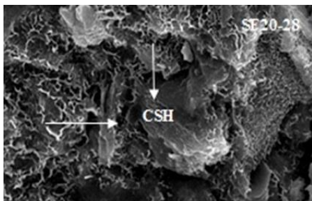
Fig-10 SEM Image for M-5 after 28 days Curing
