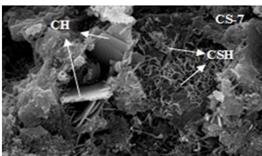
Fig-1 SEM Image for M-1 after 7 days Curing
