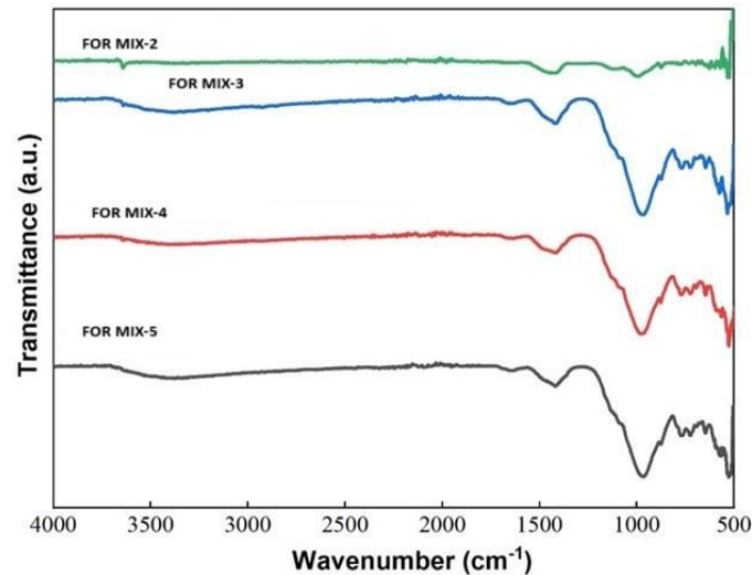
Graph-2 FTIR Observations on different Mixes
