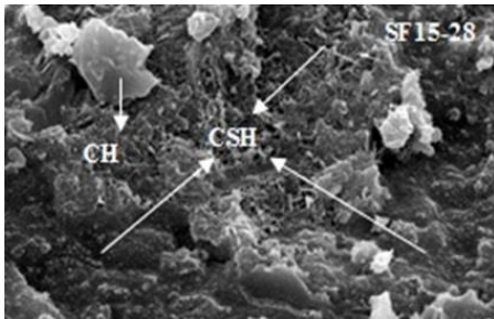
Fig-9 SEM Image for M-4 after 28 days Curing
