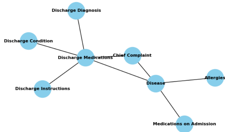
Figure 5: Knowledge Graph
