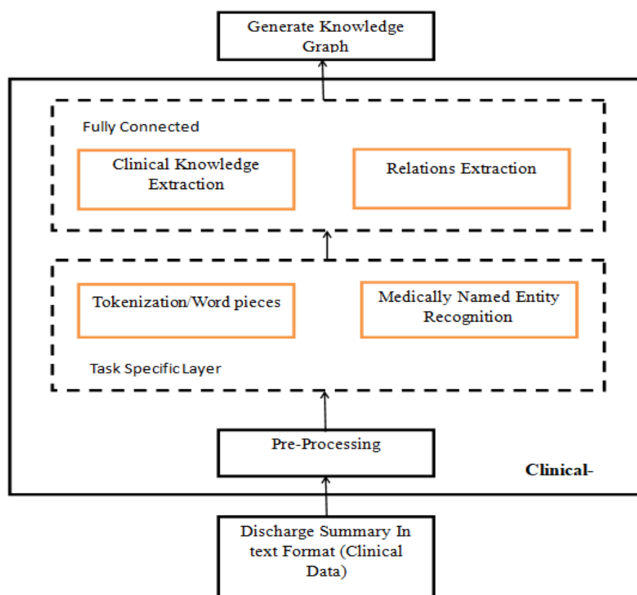
Figure 2: Architecture of our proposed model
