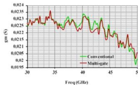
Fig. 15 Extracted g_m of two structures, ( V_{DD} = 1 V, V_{bias} = 580 mV)
