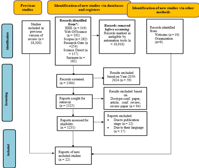
Figure 5: Prisma Model.
