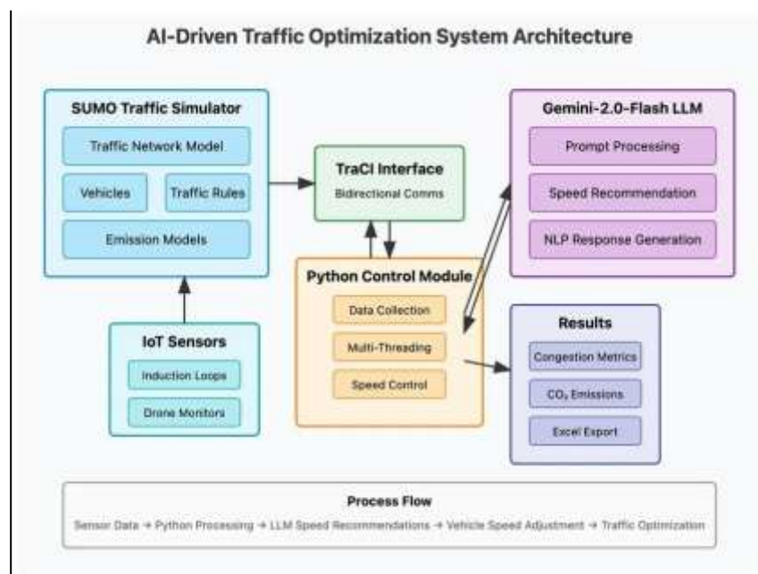
Figure 5: System architecture of the AI-driven traffic optimization framework
