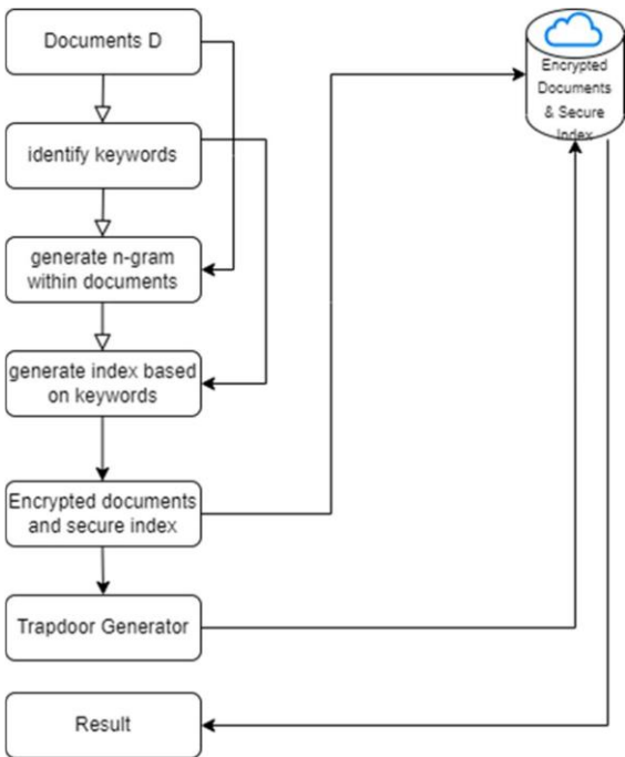
Fig. 3 Proposed Flow
