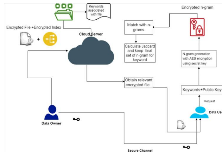
Fig. 2 Proposed architecture
