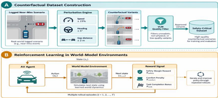
Fig. 2. Integrated workflow for counterfactual dataset construction (top) and reinforcement learning in world-model environments (bottom): near-miss logs are perturbed and quality-filtered to build safety-critical training sets, while the world model serves as the environment for policy optimization through reward-driven rollouts.
