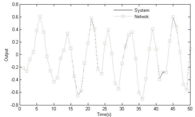
Figure 4. Response of the system ( RMSE error= 5.33145E-03)
