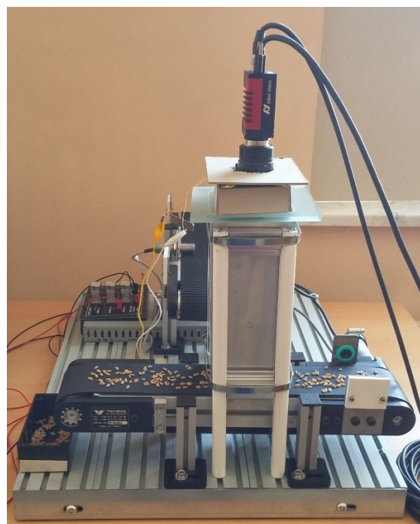
Figure 2. Dynamic system used for acquiring video sample of durum wheat grains with impurities
