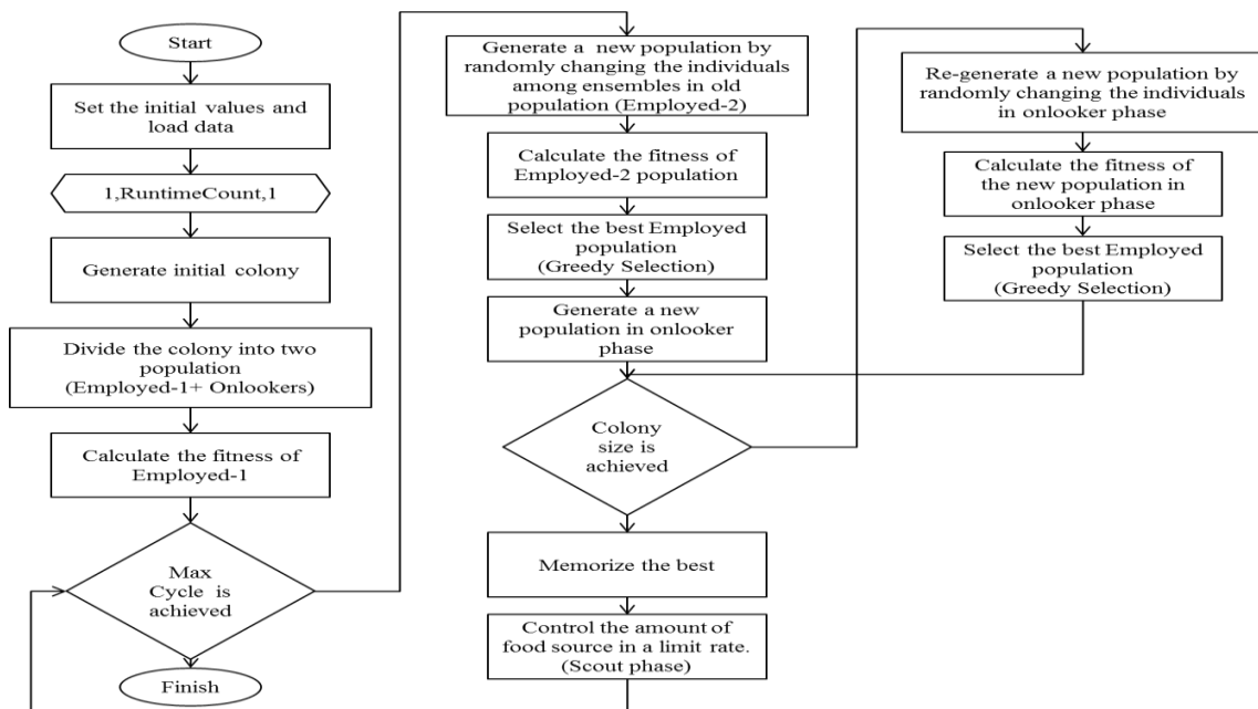
Figure 5. Flow chart of the proposed algorithm
